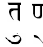
Classifier output
