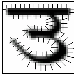
192 gradient features with gradients quantized in 12 directions
