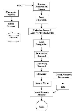
Figure 3: Answer Processor Architecture.
