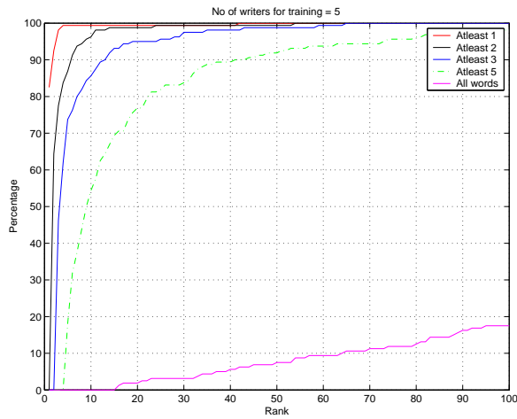
(a) Recall with 5 writers for training.
