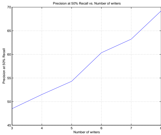
Figure 16. Precision at 50% recall is plotted against different numbers of writers used for training. As more number of writers are used for training, the precision at a given recall increases.
