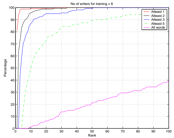
(b) Recall with 6 writers for training.
