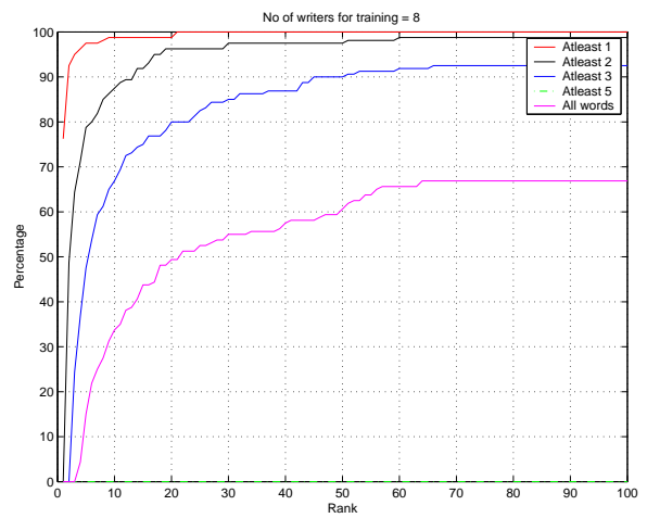
(b) Recall with 8 writers for training.
