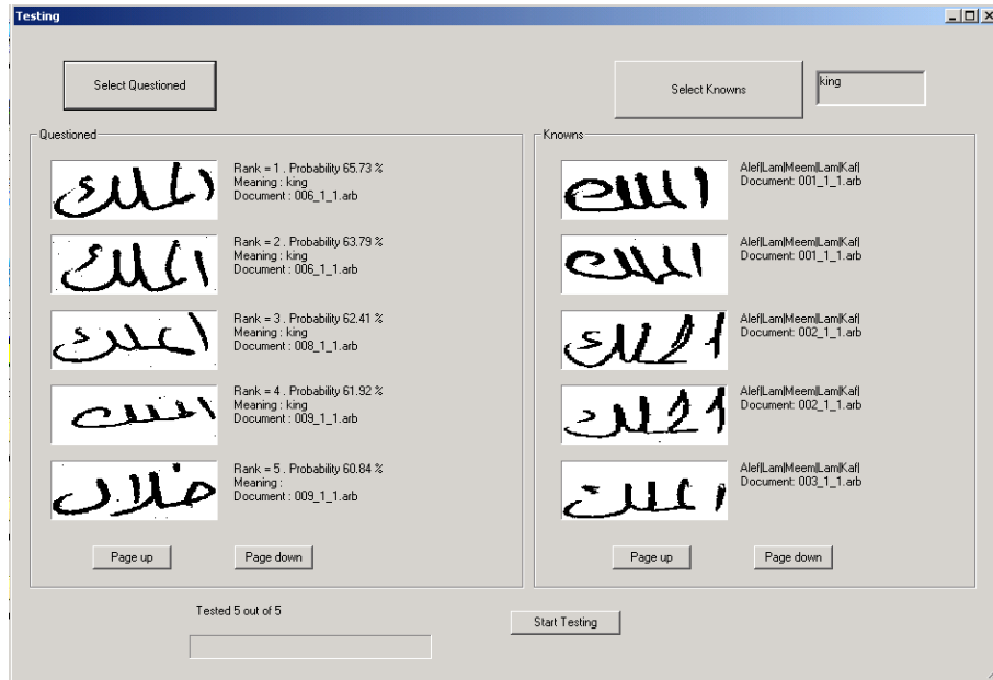
Figure 3. Word spotting results. The template word images on the right side, obtained in the first step, are used to spot the images shown on the left. The results are sorted in rank by probability. The images on the right are the selected prototypes and those on the left are the ranked set of test images.
