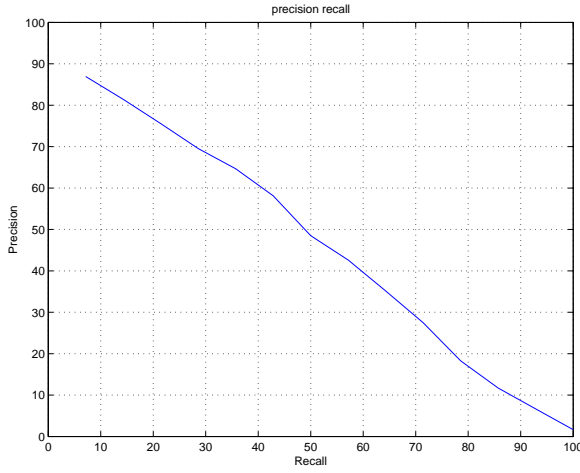
(a) Precision Recall with 3 writers for training.
