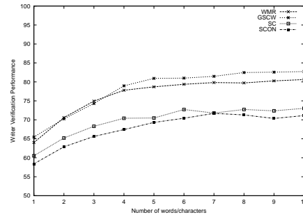
Figure 2. Verification accuracy for accumulated words
