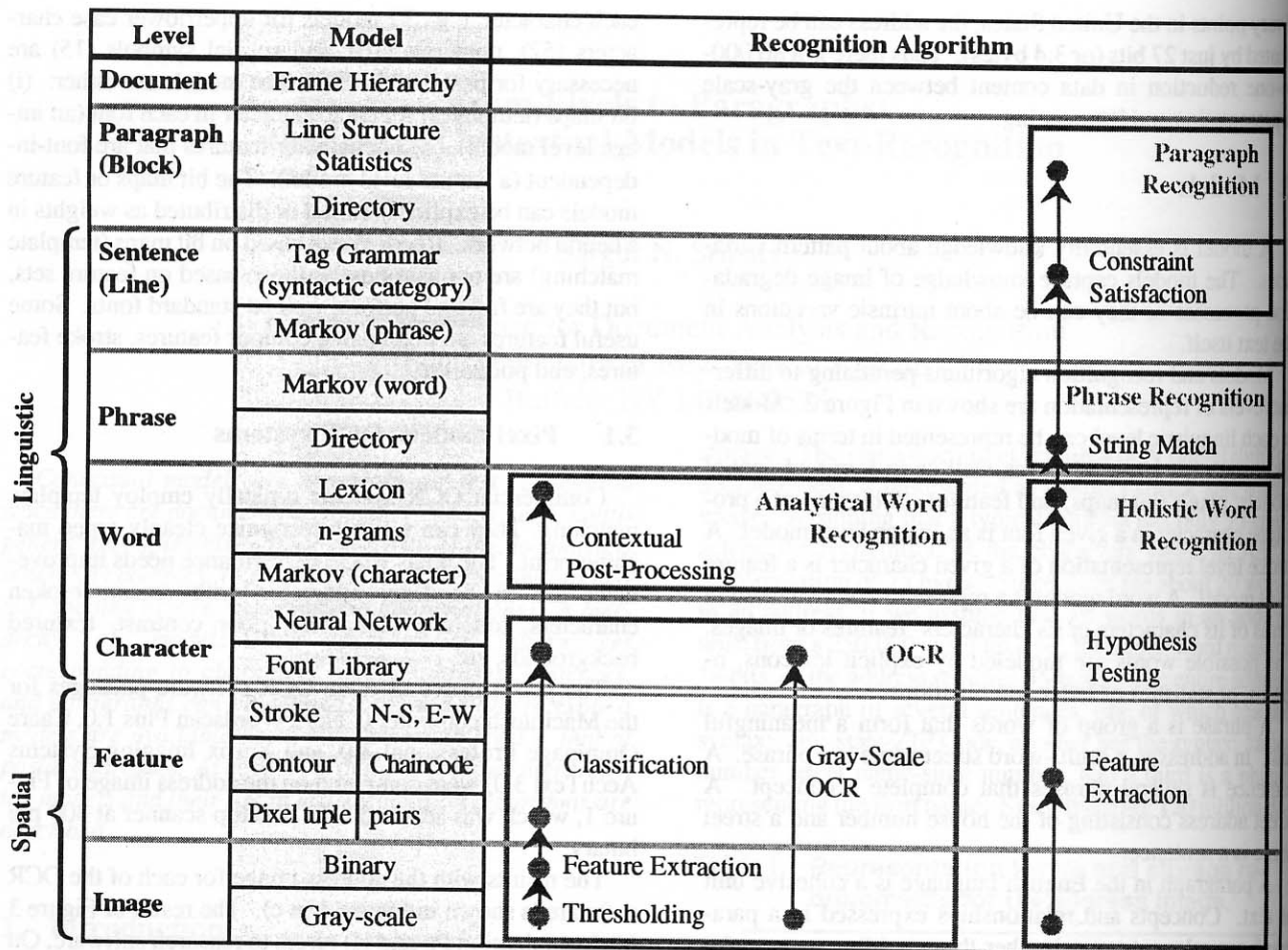
Figure 2. Hierarchy of levels, models, and algorithms in text recognition.
