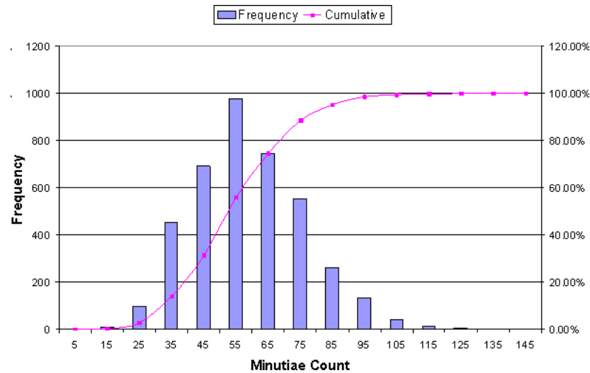
Fig. 3. Distribution of detected minutiae count for an image area of 1.95cm x 2.93cm.
