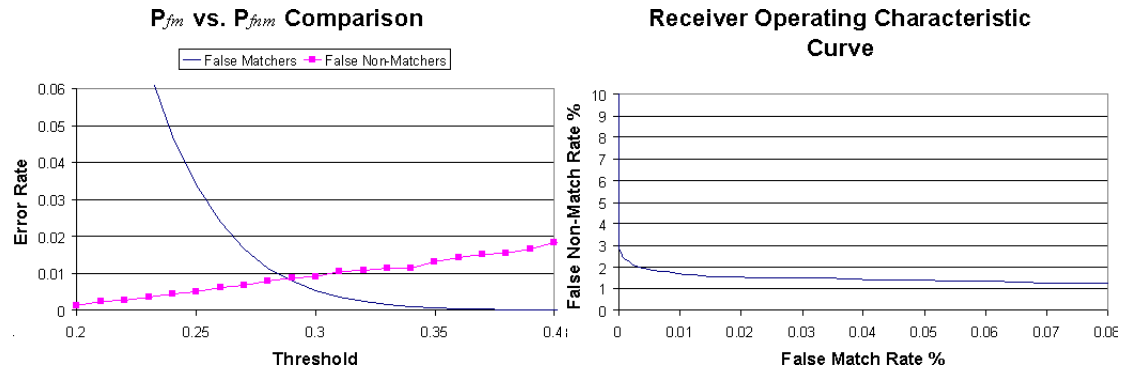
Fig. 4. Error rate versus match score distribution for an image area of 1.95cm x 2.93cm and corresponding ROC curves.
