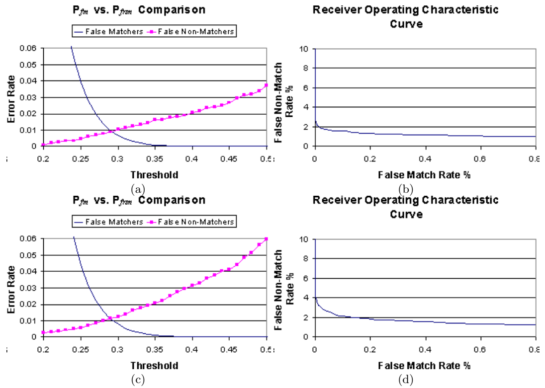
Fig. 5. Error rate versus match score distribution for an image area of 1.9cm x 1.9cm (and corresponding ROC curves) created by cropping (a and b) and centroiding (c and d).
