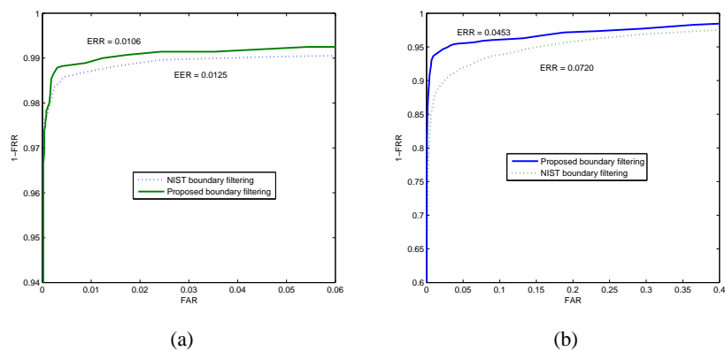
Fig. 6. ROC curves for (a) FVC2022 DB1 and (b) FVC2022 DB4.
