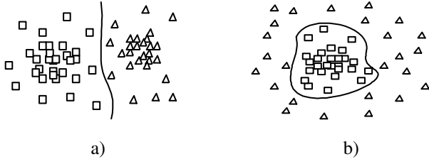
Figure 1. Two different cases of two-category classification problem. a) Regular two-category problem has two clusterings with open decision boundary. b) Signature verification is a special two-category problem with closed decision boundary around the clustering genuine signatures.
