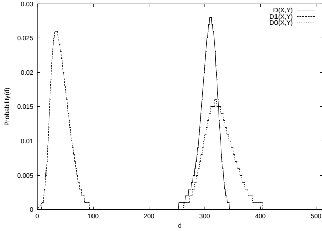
Figure 1. Distributions of D(X,Y) ( \in \phi^a ), D1 = X \odot Y , and D0 = \bar{X} \odot \bar{Y} with \beta = 0.5 , \forall X \in \mathcal{F}, \forall Y \in \mathcal{G} . Here, d represents dissimilarity value.
