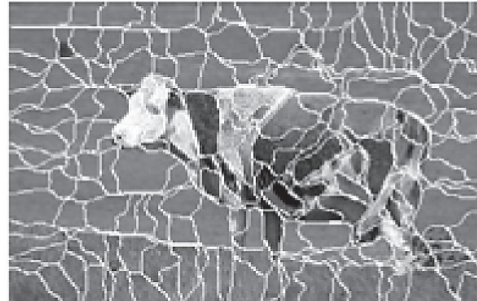
Each superpixel is a random variable
